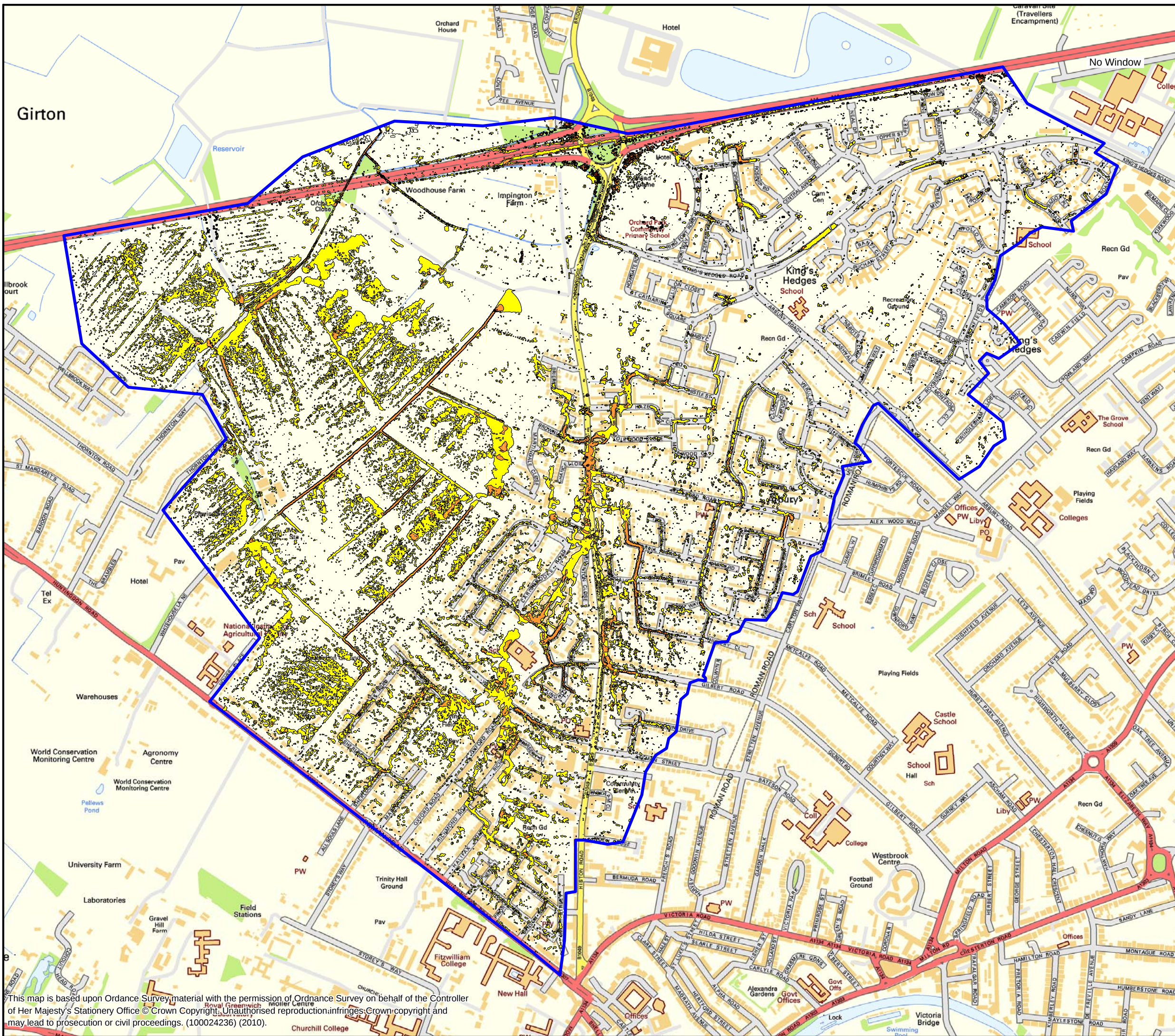
FIGURE F11 0.5% AEP "ENGINEERING OPTION C2" PLUVIAL MODELLING MAXIMUM VELOCITY - KING'S HEDGES AND ARBURY
